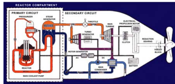
Figure 2 UK nuclear submarine layout [5]
