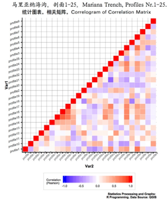
Figure 9 Cross-correlation matrix of the depth values in bathymetric profiles of the Mariana trench
