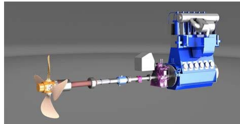
Figure 7 Shaft propeller [9]
